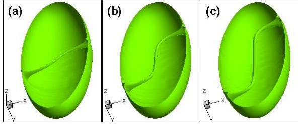
FIG. 5: Single S vortex configuration for \Omega/\omega_x = 0.38 (a), 0.44 (b), 0.48 (c).
